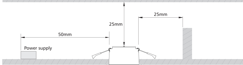
Fig 1: Installation Spacing
