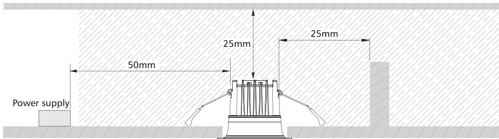
Fig 1: Installation Spacing
